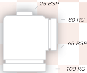
Hydrant Hose Reel Elbow
