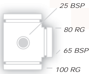
Hydrant Hose Reel Tee
